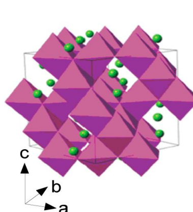
spinel \text{LiMn}_2\text{O}_4 3D
