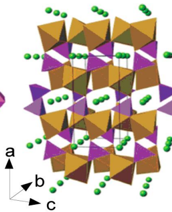
olivine \text{LiFePO}_4 1D
