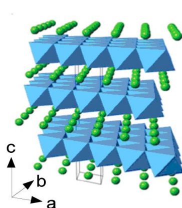
layered \text{LiCoO}_2 2D
