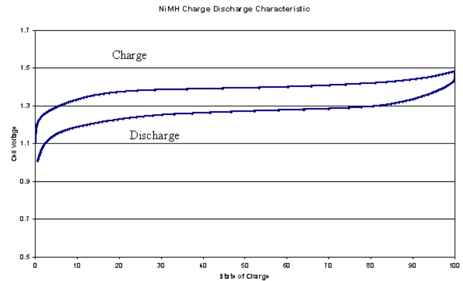
Figure 1. NiMH Charge Discharge Characteristic
