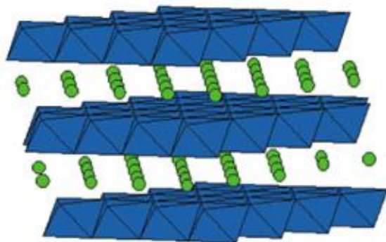
\text{LiCoO}_2 : layered structure
